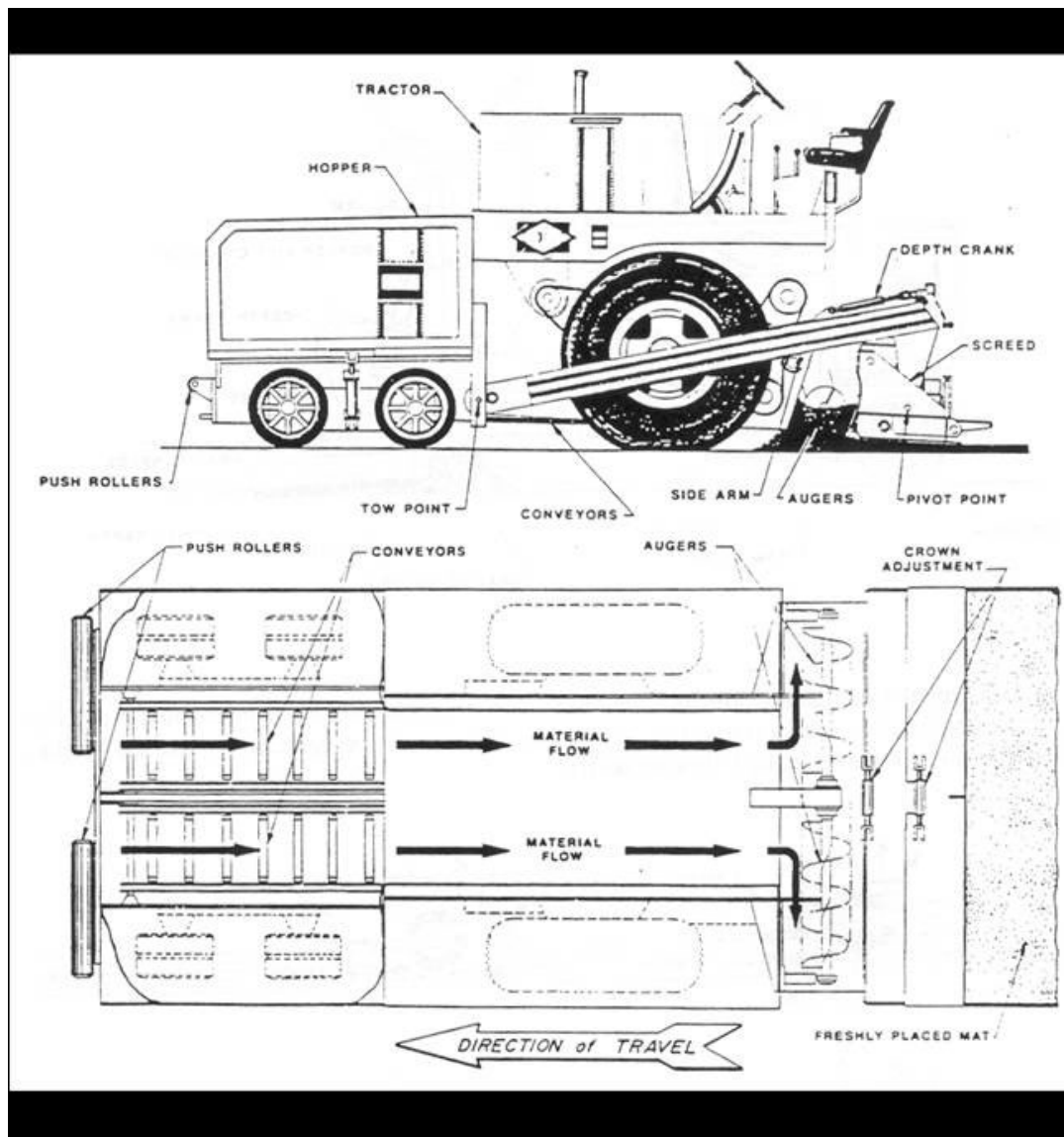
Figure 13.24-3a Asphalt Paver
